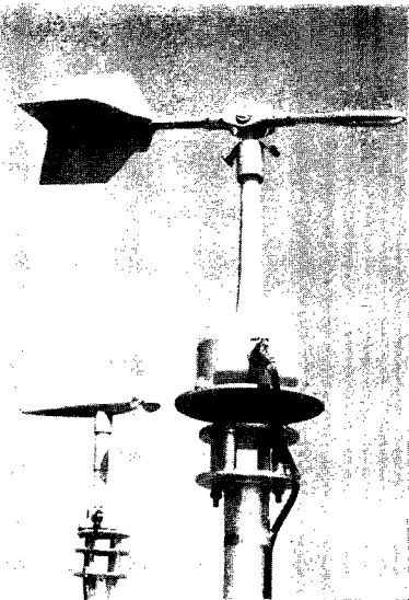
Fig. 1 A view of the new all-weather type bivane and propeller anemometer.
