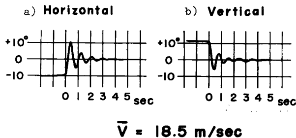
Fig. 2 Transient response of the bivane to the sudden change of wind direction in the wind tunnel.
