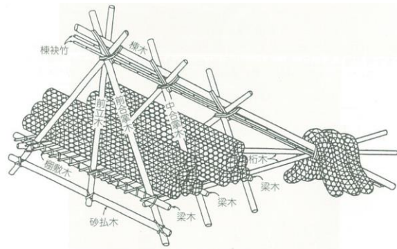
Fig. 6 Seigyū, Hijiriushi (after Home Ministry (1881))
