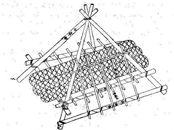
Fig. 7 Hishiushi (after Home Ministry (1881))
