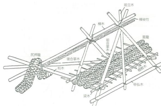
Fig. 5 Kawakura (after Tomino (2002))
