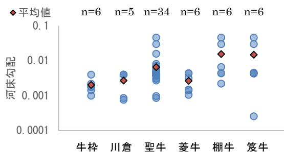
Fig. 10 Bed slope at construction points of each crib spur
