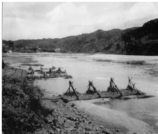
Photo 2 Seigyū (crib spur) in the Kizu River in 1953 (Photo taken by Horii. Courtesy of Nakatsugawa and Fukui)
