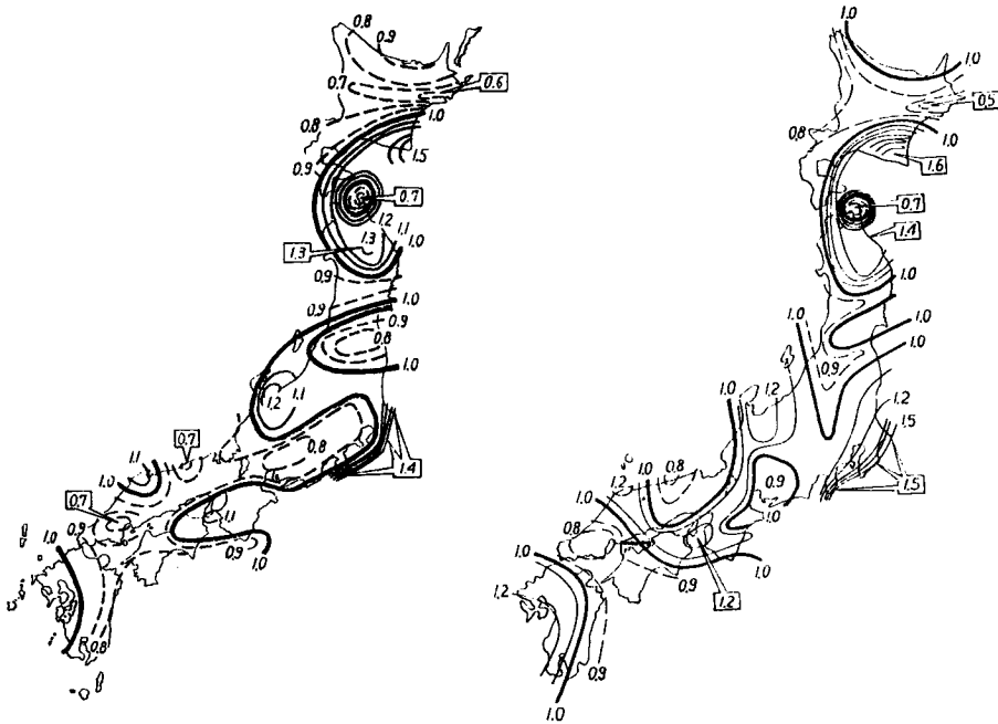
Fig. 3a S_q Anomaly in Japan, expressed by amplitude-ratios referred to value of Kakioka
