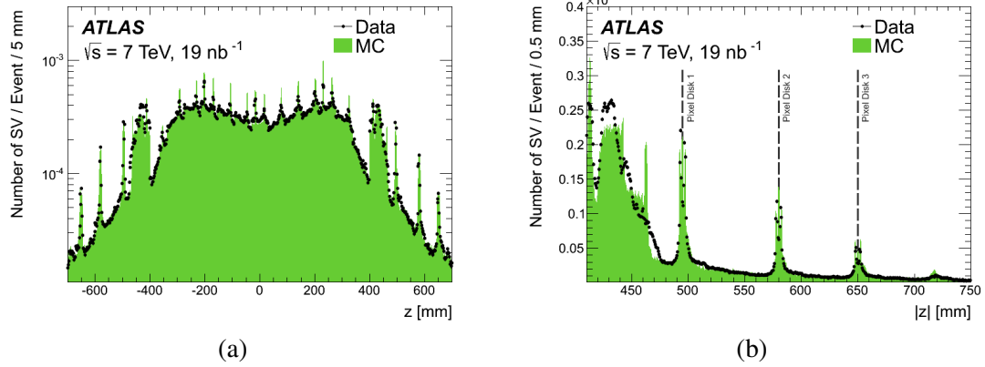
Figure 8. Number of selected secondary vertices per event in data (points) and MC simulation (solid histogram), as a function of z , (a) for |z| < 700 mm, and (b) for |z| > 410 mm, where vertices with r < 50 mm and r > 155 mm are excluded to highlight the pixel end-cap region.
