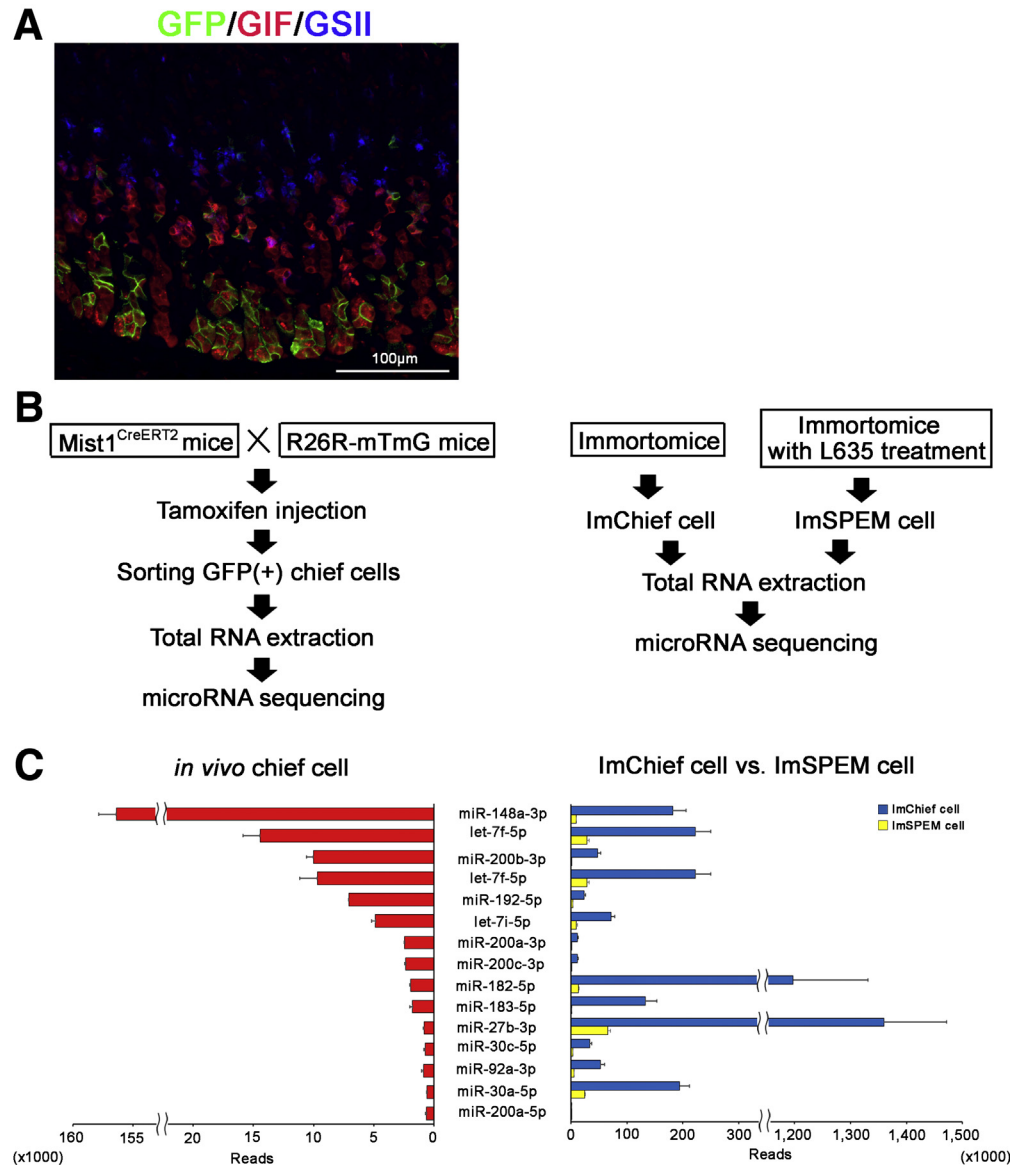
Figure 1. miRNAs related to SPEM development.
