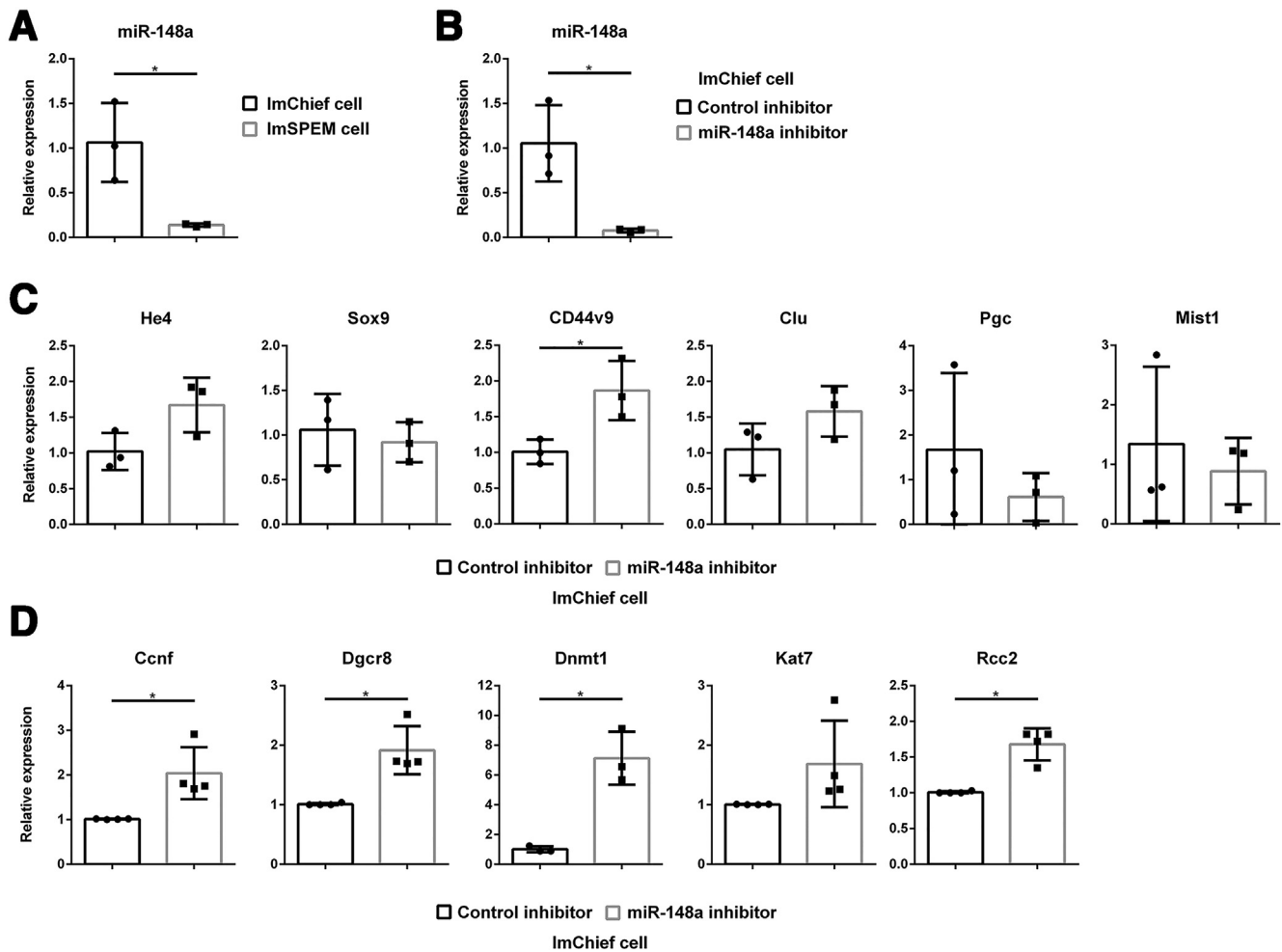
Figure 5. Involvement of miR-148a in initiation of chief cell transdifferentiation. (A) Expression of miR-148a in ImChief cells and ImSPEM cells by microRNA assay. Mann-Whitney U test, *P < .05 . (B) Expression of miR-148a by microRNA assay in ImChief cells treated with control inhibitor or miR-148a inhibitor. Mann-Whitney U test, *P < .05 . (C) Expression of genes related with SPEM cells ( He4 , Sox9 , Cd44v9 , and Clu ) or chief cells ( Pgc and Mist1 ) in ImChief cells treated with control inhibitor or miR-148a inhibitor by quantitative PCR. Mann-Whitney U test, *P < .05 . (D) Expression of miR-148a target genes in ImChief cells treated with control inhibitor or miR-148a inhibitor by quantitative PCR. Mann-Whitney U test, *P < .05 .
