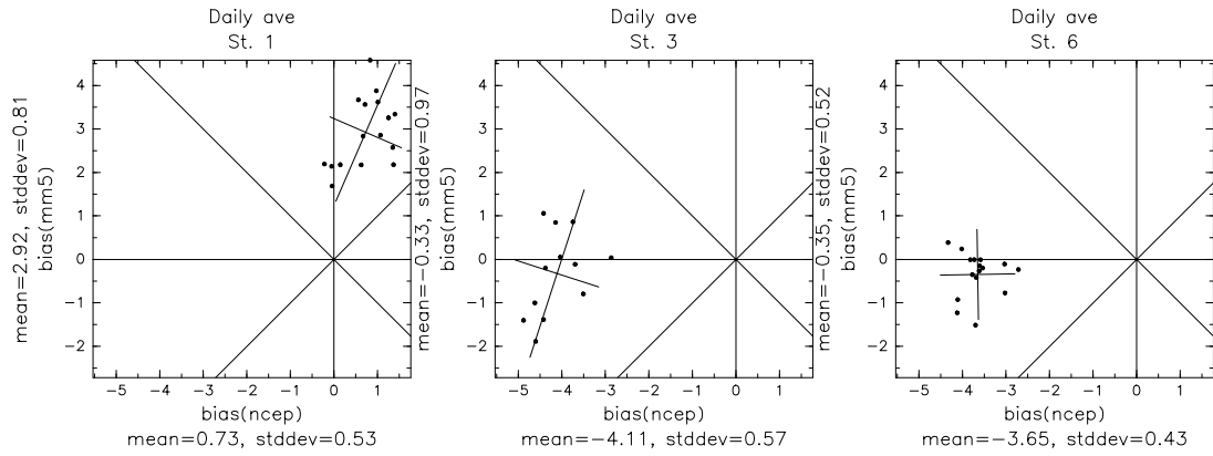
Fig. 5. Bias of the NCEP FNL and MM5 for station no. 1, 3, and 6.
