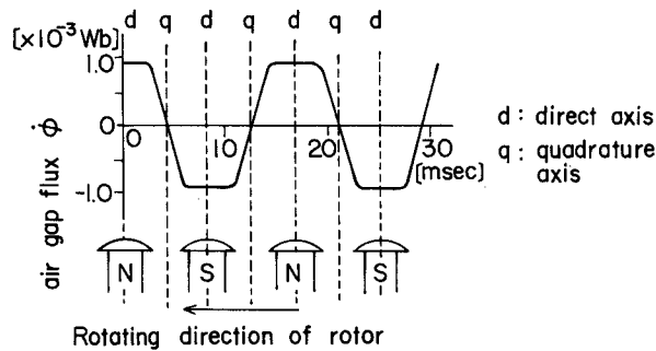
Fig. 9 Air gap flux waveform and pole position at no-load
