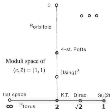
図 2: (c, \bar{c}) = (1, 1)
