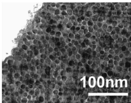
FIG. 2. Plane view TEM image taken from as-deposited \text{ZnFe}_2\text{O}_4 thin film.
