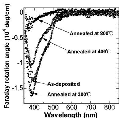
FIG. 4. Faraday rotation angle as a function of wavelength for as-deposited (open circles) and annealed \text{ZnFe}_2\text{O}_4 thin films. The annealing temperature is 300 (closed circles), 400 (open triangles) and 800 °C (closed triangles).
