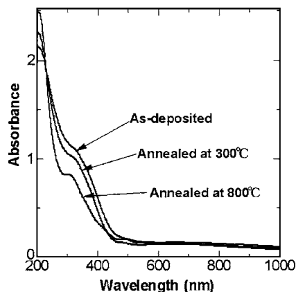
FIG. 3. Optical absorption spectra for as-deposited and annealed \text{ZnFe}_2\text{O}_4 thin films. The annealing temperature is 300 and 800 °C.
