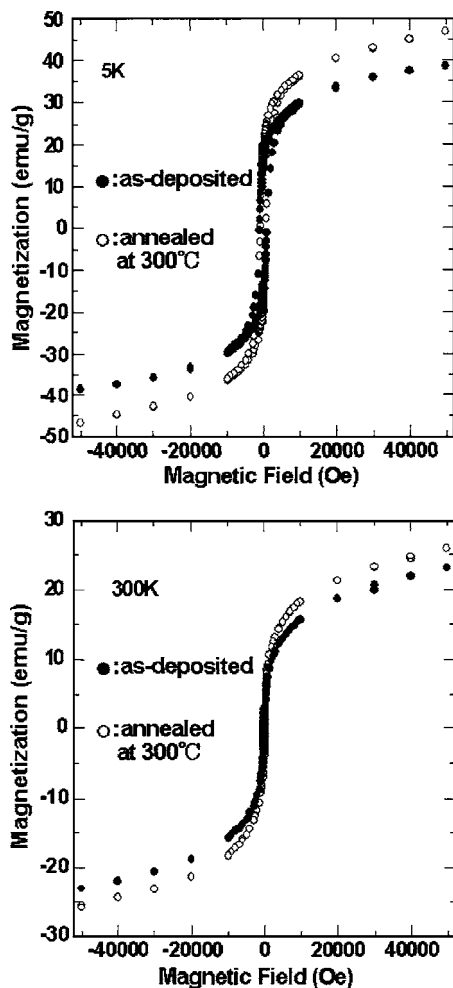
FIG. 1. Dependence of magnetization on external magnetic field at 5 and 300 K for as-deposited (closed circles) and annealed (open circles) \text{ZnFe}_2\text{O}_4 thin films prepared by the sputtering method. The annealing temperature is 300 °C.
