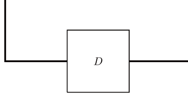
Figure 5: A diagram D of F
