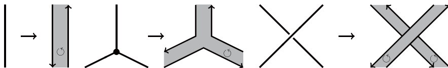
Figure 2: A construction of F(D)
