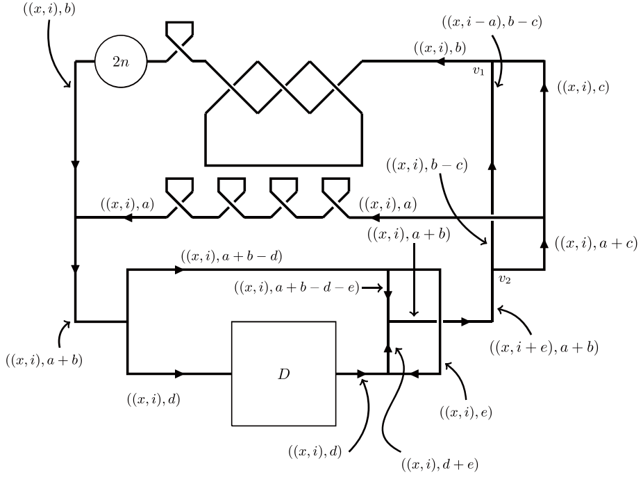
Figure 8: X -colored diagram D'_n
