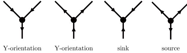
Figure 3: Orientations around vertices
