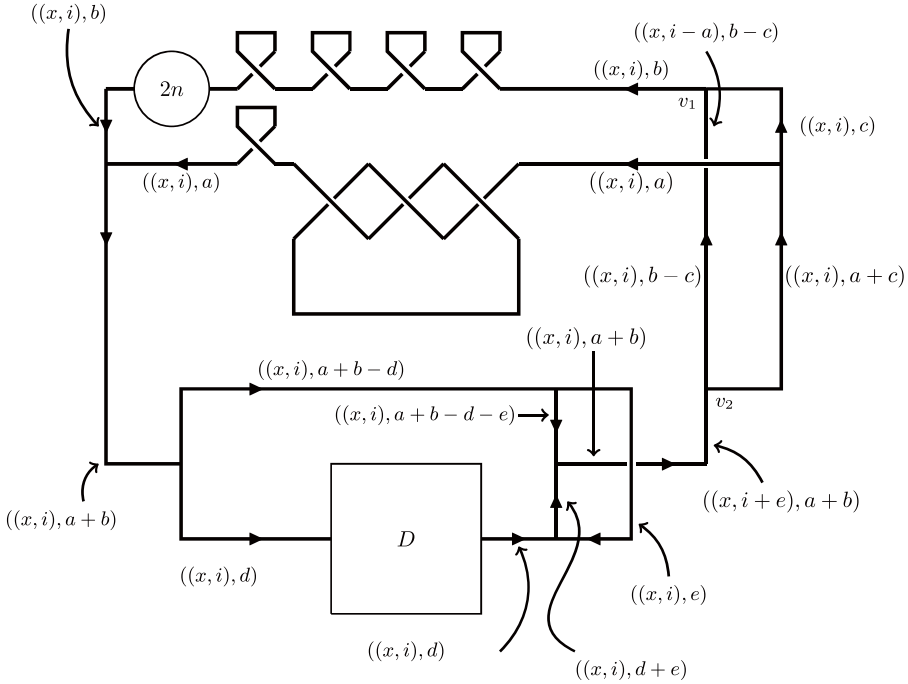
Figure 7: X -colored diagram D_n
