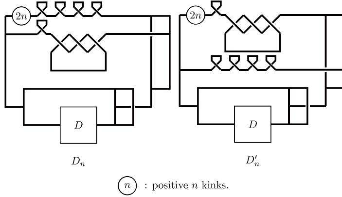
Figure 6: Diagrams D_n and D'_n ( n \in \mathbb{Z}_{\geq 0} )
