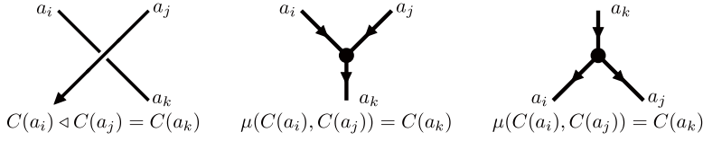
Figure 4: Coloring conditions at crossings or vertices
