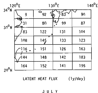
Fig. 8. Distributions of sensible and latent heat fluxes in July.
