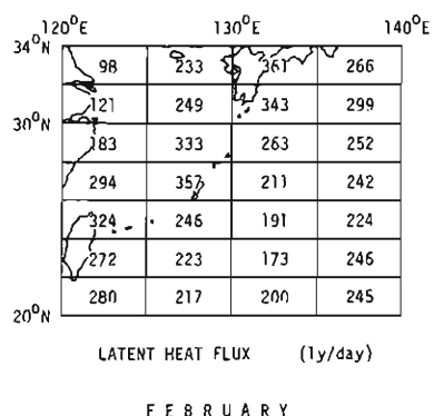
Fig. 7. Distributions of sensible and latent heat fluxes in February.
