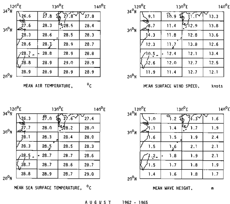
Fig. 3. Monthly means of marine meteorological parameters in August.
