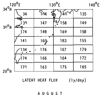
Fig. 9. Distributions of sensible and latent heat fluxes in August.
