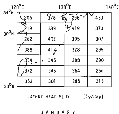
Fig. 6. Distributions of sensible and latent heat fluxes in January.
