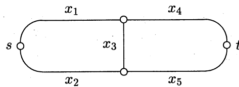
Figure 1: The graph G_f representing a path function f = x_1 x_4 \vee x_2 x_5 \vee x_1 x_3 x_5 \vee x_2 x_3 x_4 .
