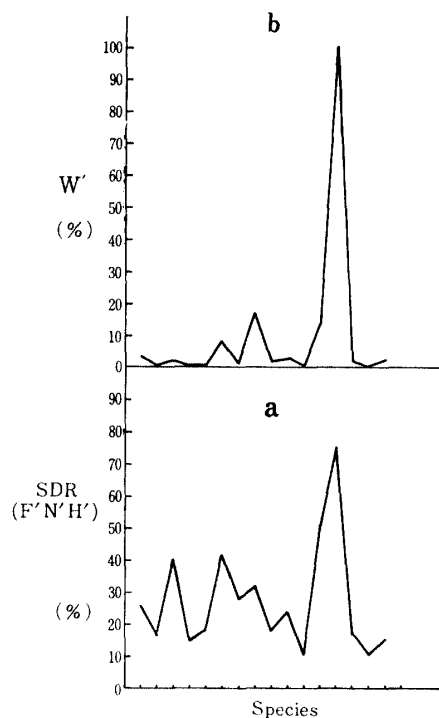
Fig. 6 Composition curve of the ground vegetation (plants less than 1.3 m in height) in SP. a-SDR by F' , N' and H' , b- W' , c-a/species No., b/species No. Species order is the same as Table 6
