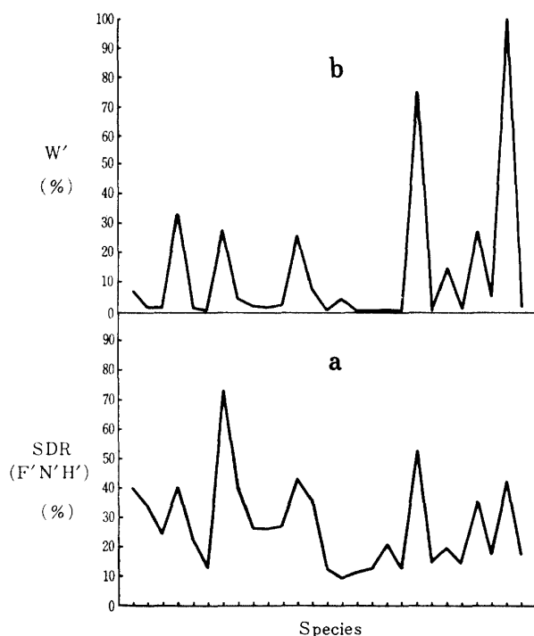
Fig. 5 Composition curve of ground vegetation (plants less than 1.3 m in height) in KBP. a-SDR by F' , N' and H' , b- W' , c-a/species No., b/species No. Species order is the same as Table 4.
