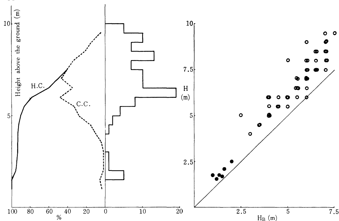
Fig. 4 Crown depth diagram and H-H_B relation in SP
