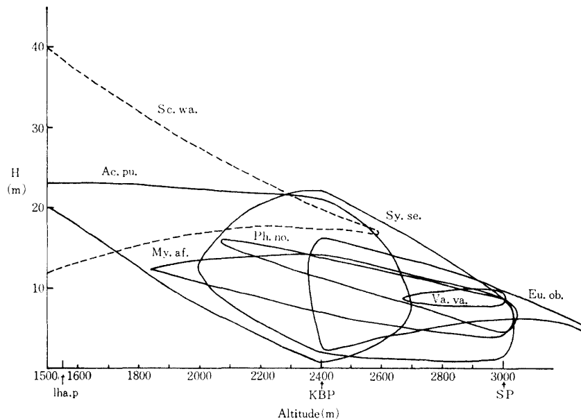
Fig. 7a Schematic sketch of the distribution of the main species occur in KBP and SP. Some of the connected species in the 1 ha. plot are also included.
