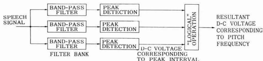
Fig. 2 Schematic diagram of the pitch extractor.
