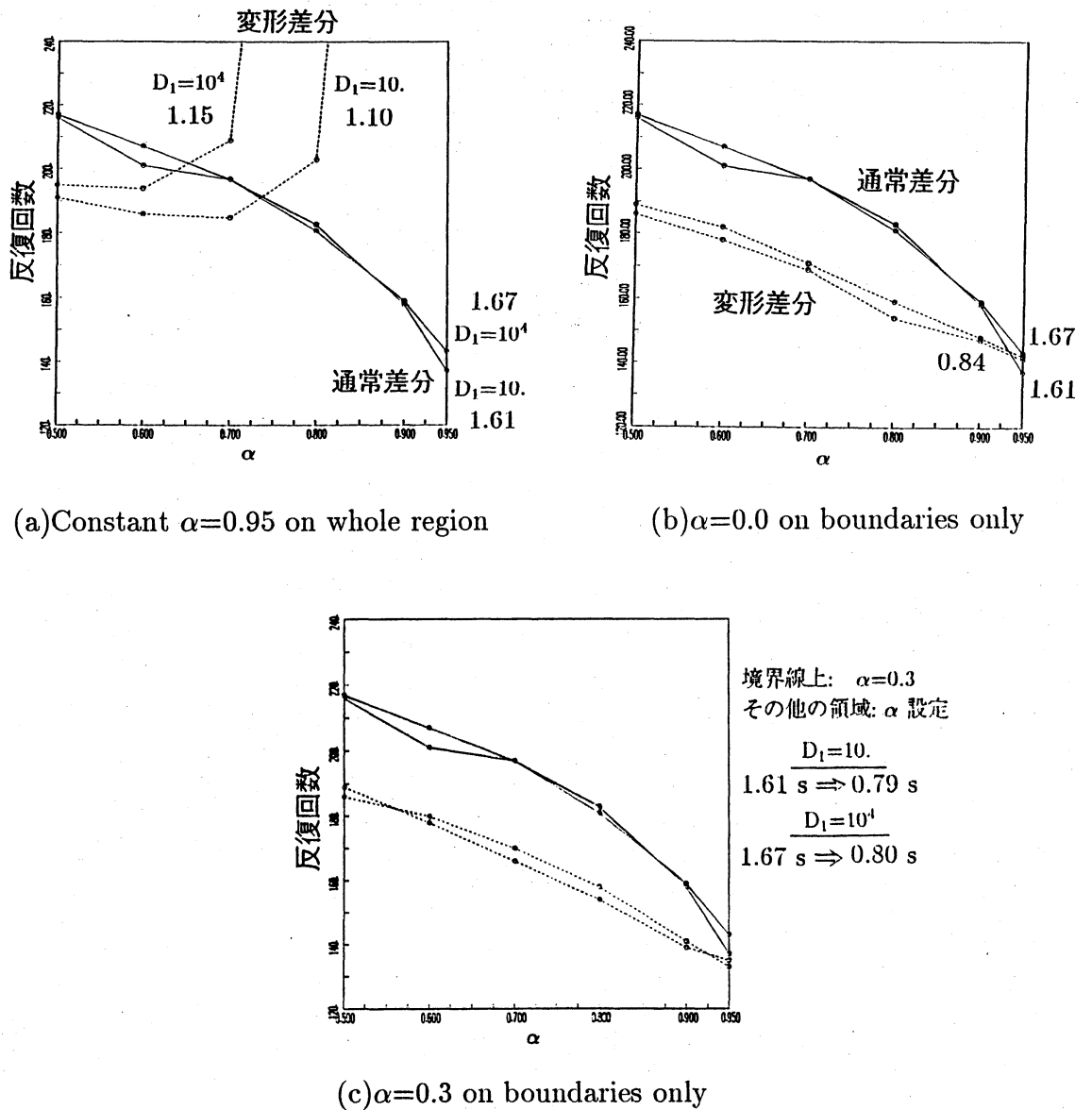
Fig. 7. Convergence property of MICCG method using a variant of difference scheme
