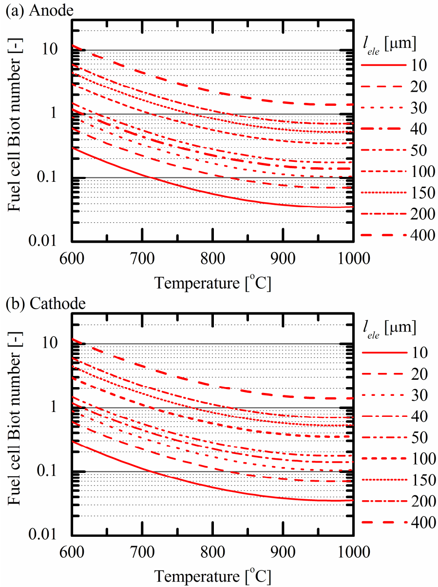
Fig. 1.2 Temperature and electrolyte thickness dependences of fuel cell Biot number at a current density of 300 mA/cm 2 .
