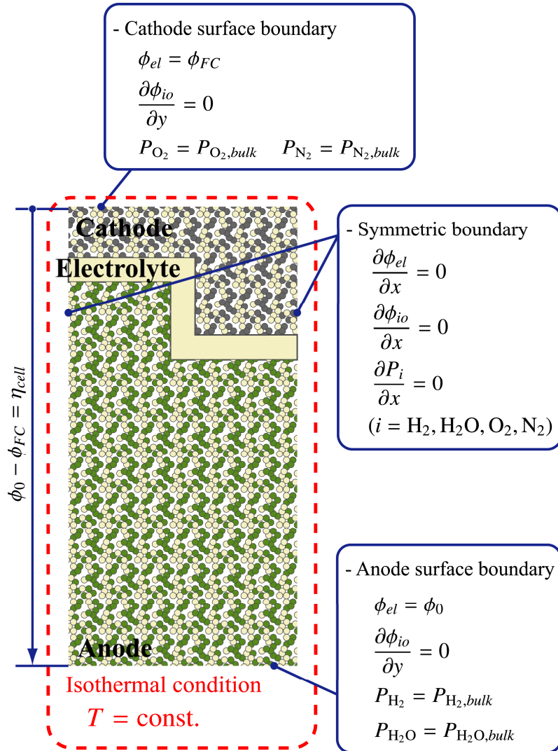
Fig. 4.4 Calculation and boundary conditions.
