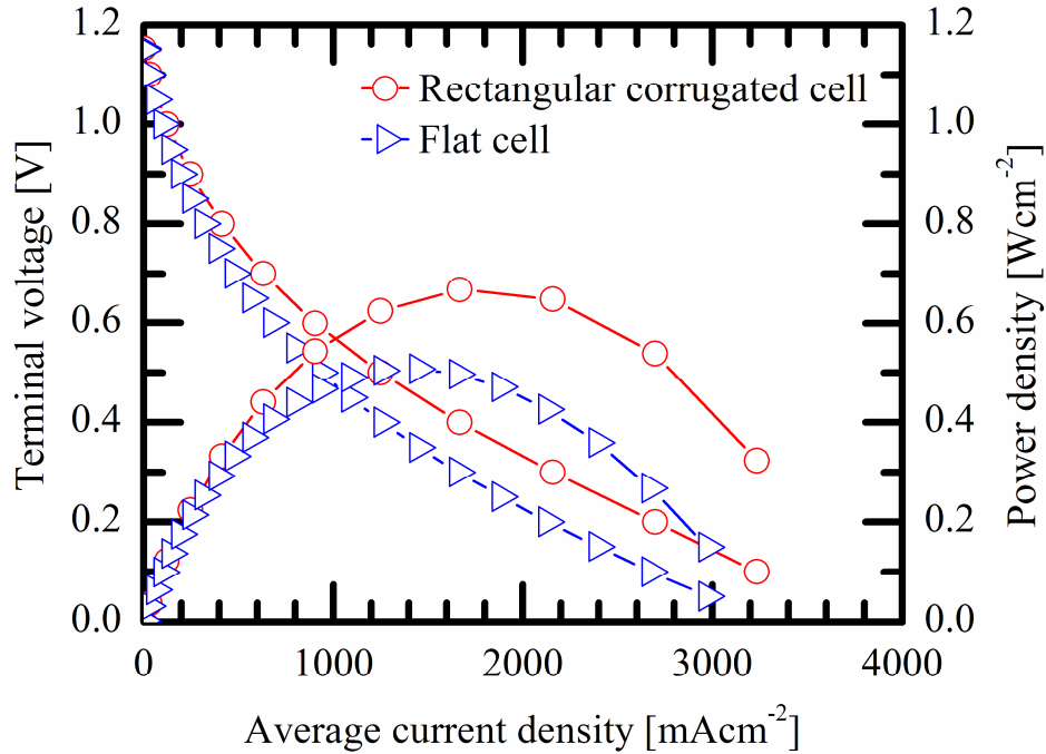
Fig. 4.10 Characteristics of i - V and i - P for Case 4.
