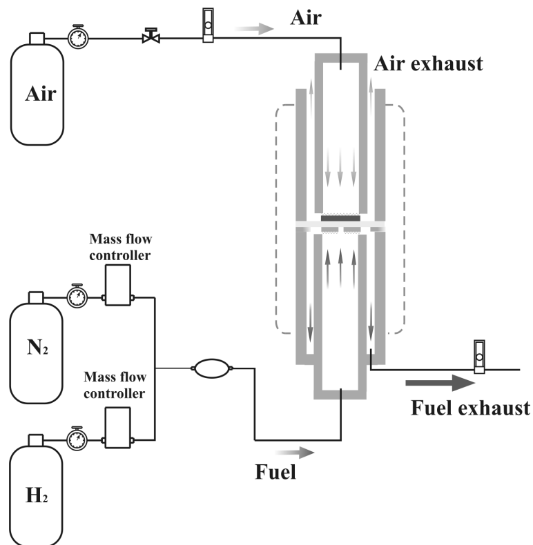
Fig. 3.5 Experimental apparatus used for power generation test involving button-type cell.
