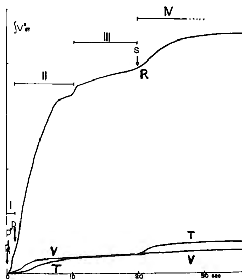
Fig. 7. Picture of \int_0^\infty v_i^2 dt , each phases are referred to the result of Miboro Explosion.
