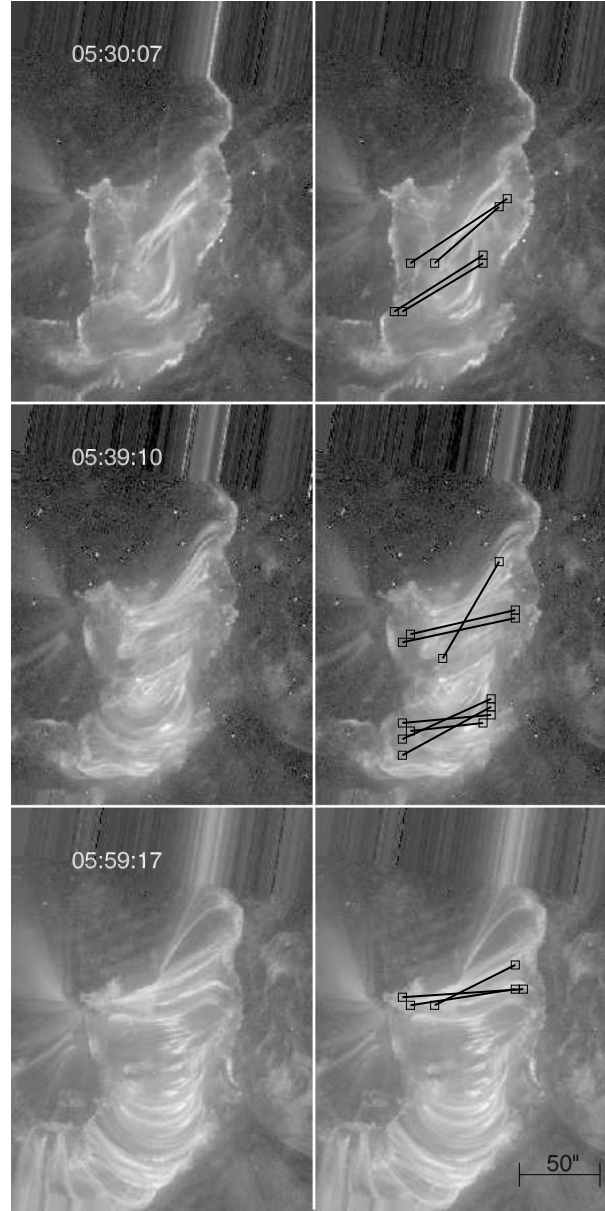
Figure 2.5: Comparison of the spatial configuration between the highly correlated pairs of the H \alpha kernels and the post-flare loops seen in the TRACE 171 Å. Celestial north is up, and west is to the right. Left panels : TRACE 171 Å images. Right panels : TRACE 171 Å images overlaid with the solid lines that connect some highly correlated pairs of H \alpha kernels.
