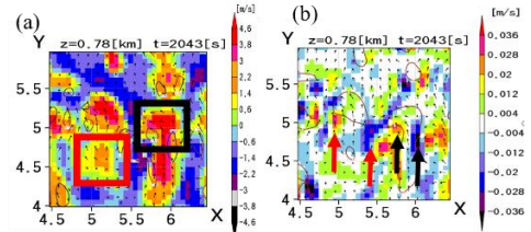
Fig. 8 (a)Vertical velocity at horizontal plane (b)Vorticity at horizontal plane
