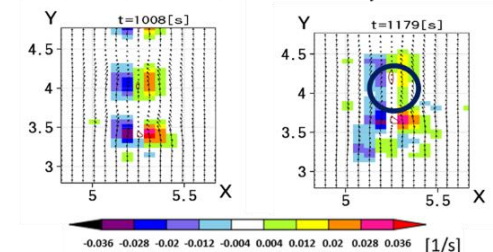
Fig. 4 Aggregation in southern surface area
