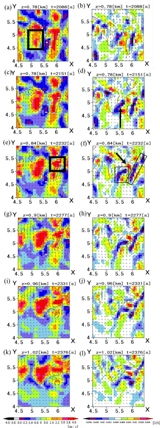
Fig. 9 Vertical velocity and Vorticity at horizontal plane
