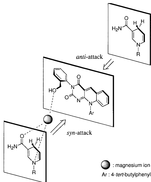
Figure 1. Most predominant intermolecular arrangements between (S)-(+)- 1 and an NAD(P)H analog at the transition states of (net) hydride-transfer reactions in the presence ( syn face) and absence ( anti face) of magnesium ion, respectively. The conformation of the side-chain carbamoyl group of NAD(P)H analog is drawn arbitrarily.
