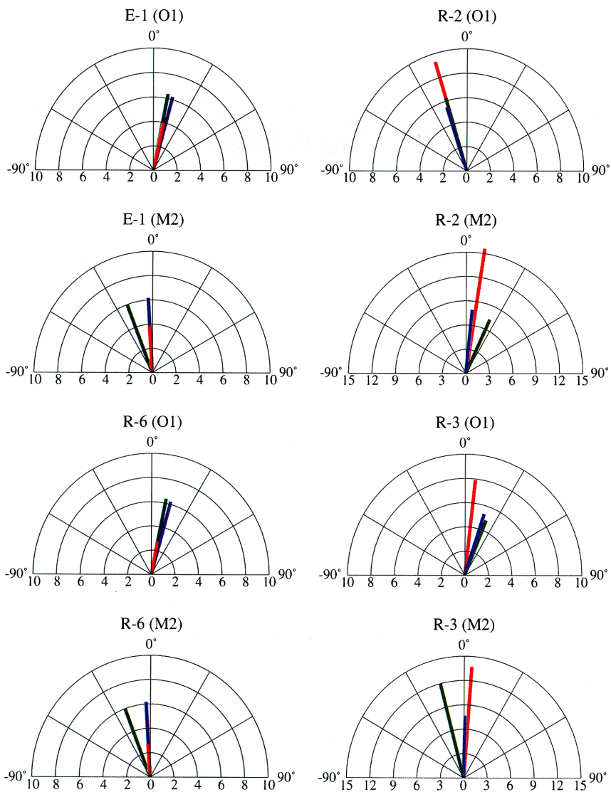
Fig. 3 Phasor diagrams of tidal factor. The center is \text{lag}=0^\circ , and right side is phase lag. Green, blue, and red lines are solid earth tide, theoretical tide including ocean loading effect, and observed tide, respectively. The ocean loading effect is not present, but it is apparent that subtracting the solid earth tidal vector from the theoretical tidal one.
