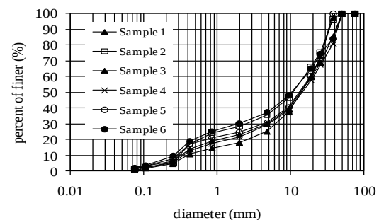
Fig. 3 Grain size of Sesayap River at Malinau
