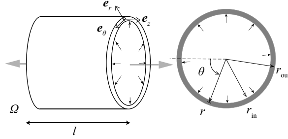
(c) Application of external loads. Current configuration \Omega . Loaded deformed state. The set \{e_r, e_\theta, e_z\} is the local covariant basis of the cylindrical coordinate system. The contravariant components of a spatial point vector are denoted as (r, \theta, z) .
