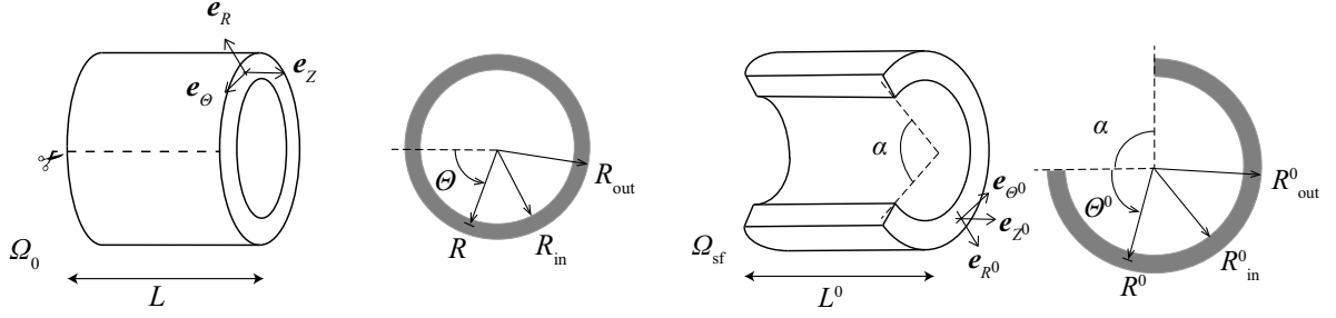
(a) Arterial segment excised from the body. Reference configuration \Omega_0 . Closed load-free state. The set \{e_r, e_\theta, e_z\} is the local covariant basis of the cylindrical coordinate system. The contravariant components of a material point vector are denoted as (R, \Theta, Z) .
