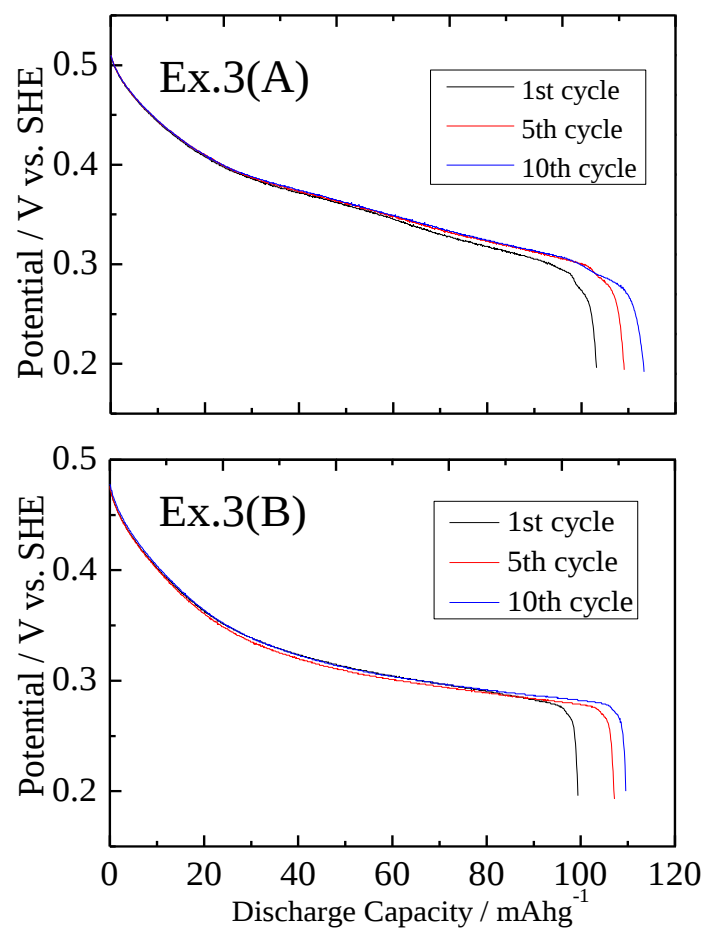
Fig. 2-12 Discharge curves for the full charge-discharge cycles in Ex.3(A) of 40 – 60 % of SOC region and Ex.3(B) of 20 – 40 % of SOC region for nickel mesh CC.
