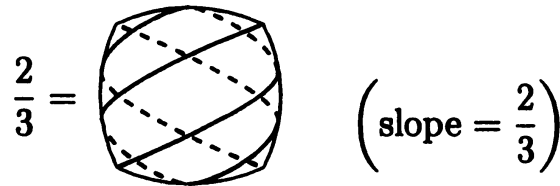
Figure 3: The rational tangle 2/3
