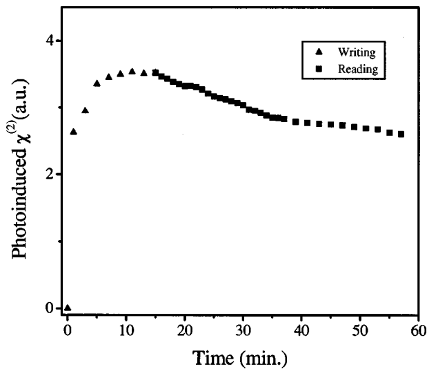
FIG. 1. Growth and decay processes of the photoinduced \chi^{(2)} of a 73\text{ }\mu\text{m} film.
