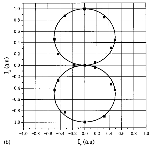
FIG. 3. Photoinduced \chi^{(2)} symmetry of a 73\text{ }\mu\text{m} film by nonresonant dual-frequency coherent excitation. (a): tensor data and fits for the x component of SHG signals from the photoinduced \chi^{(2)} ; (b): the data were obtained by simultaneous rotation of the input-beam polarization and the analyzing polarizer.
