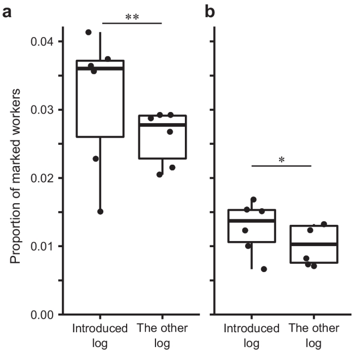
Figure 2 Comparison of the proportion of marked workers between the logs in which they were introduced and the other log in the two-week (a) and 4-week test period group (b). Asterisks indicate significant differences (likelihood ratio test, *p < 0.05 , **p < 0.01 ).
