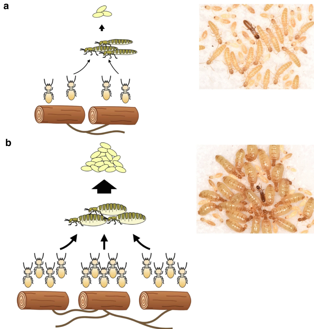
489 Figure 1 Schematic representation of the nutritional contribution of workers on egg production in 490 small ( a ) and large colonies ( b ). A single colony uses multiple logs which are connected by tunnels. 491 Even if the workers forage from multiple logs, the nutrients necessary for egg production are 492 concentrated in the queens, so the number of eggs produced is likely to reflect the number of workers 493 in the colony. The size of the queens varies remarkably among colonies.
