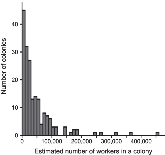
525 Figure 5 Histogram of colony size in Reticulitermes speratus in the field. The x-axis represents the 526 estimated number of workers in each colony, and the y-axis represents the number of colonies. The 527 colony sizes were estimated for 188 field colonies. The estimated number of workers in a colony 528 ranged from 10,700 (first quartile) to 24,500 (median) to 58,600 (third quartile) to 451,800 529 (maximum).
