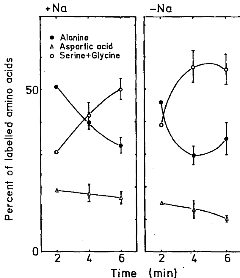
Fig. 5. Distribution of ^{14}\text{C} in the basic fraction from the leaves of Amaranthus tricolor grown with or without Na. The basic fraction: alanine (●), aspartic acid (▲) and serine plus glycine (○), were separated as described in 'Materials and Methods'. Samples were the same as those in Fig. 4. Data are the means and SD of four replicates.
