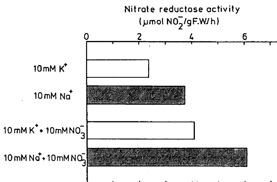
Fig. 5. Effect of Na- or NO_3^- -loading via xylem stream on the NR activity level of the cut shoots of Amaranthus tricolor . The 30-d-old Na-deficient A. tricolor seedlings were excised at about 5 mm above the root/shoot junction and the cut ends of the shoots were dipped in the test solution containing either 10 mM NaCl or 10 mM NaCl plus 10 mM KNO_3 , and in the reference treatments, 10 mM KCl or 10 mM KCl plus 10 mM KNO_3 was supplied. After 10 h under continuous illumination, the youngest fully expanded leaves were harvested from ten different shoots from each treatment and extractable NR activities were determined.
