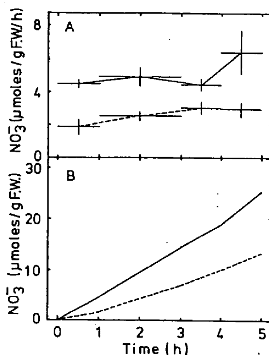
FIG. 1. Effects of Na + application on NO 3 - uptake of A. tricolor seedlings. The 30-d-old Na + -deficient A. tricolor seedlings were placed in the uptake solution supplemented with either 0.5 mM NaCl or 0.5 mM KCl at the end of the dark period (at time 0 h). A, Changes in the NO 3 - uptake rates with time; B, cumulative NO 3 - uptake. Results are represented by solid lines for the Na + -treated seedlings and by dotted lines for the K + -treated seedlings. Data are the means and SD of three replications of each four plants and are expressed as \mu\text{mol g}^{-1} root FW.
