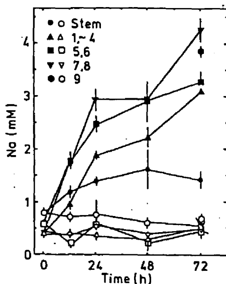
FIG. 2. Changes in the sodium concentration of leaves and stems of 30-d-old A. tricolor seedlings during the recovery from sodium deficiency. Leaf position was counted from the base to the tip of the shoot. The seedlings were supplied with 0.5 mM NaCl (●) or 0.5 mM KCl (○) at the end of the light period (at time 0 h). Data are the means and SD of determinations of four individual plants. SD are not shown when smaller than the symbols.
