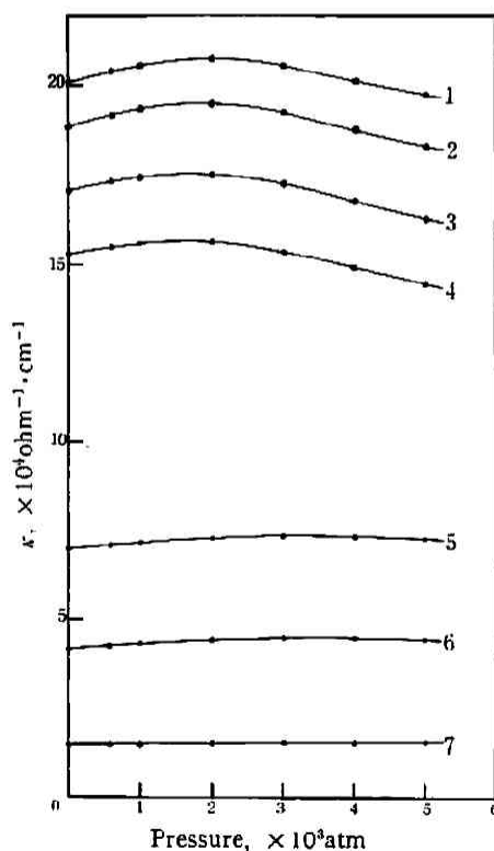
Fig. 2 Specific conductivity of DBAC at 45°C 1: 0.0236 (molal), 2: 0.0215, 3: 0.0185, 4: 0.0154, 5: 0.0051, 6: 0.0031, 7: 0.0010
