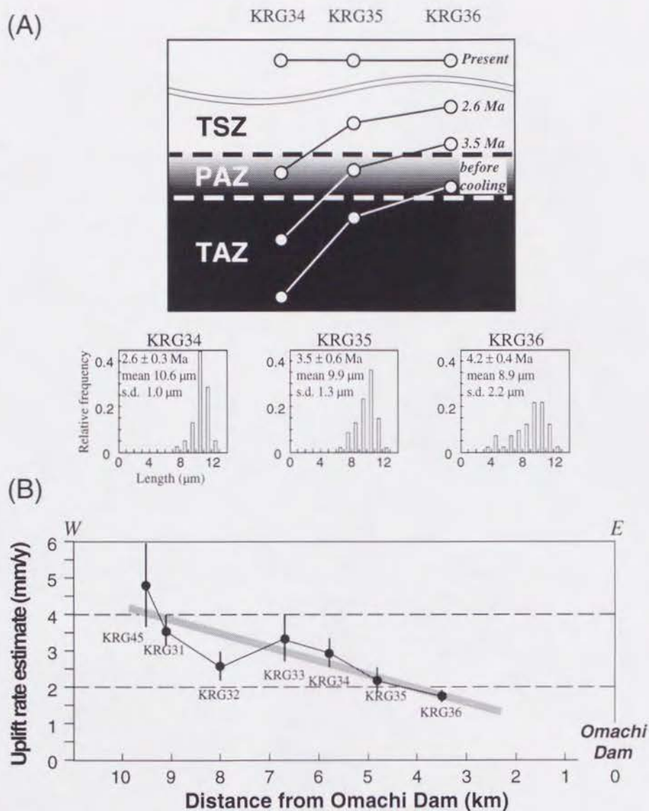
Fig. 16. (A) Schematic diagram of past position of samples of KRG34, KRG35 and KRG36 in terms of PAZ, together with the track length histograms. Apparent age ( 1\sigma ), mean track length and the standard deviation ( s.d. , 1\sigma ) are given. The histogram of KRG36 with many shorter tracks indicates that this sample should have suffered the temperature within the bounds of PAZ before uplifting. The skewed pattern of KRG34 and KRG35 indicate that these samples were located in TAZ before uplifting and passed PAZ at a certain rate after uplift started. (B) First order estimates of uplift rate of samples with "younger" ages along Transect C where initial geothermal gradient was assumed 40 °C/km. Uplift rates of each samples were obtained by dividing the depths which correspond to the middle of ZPAZ by their apparent ages, indicating the minimum estimates. Horizontal axis is the distance from the Omachi Dam. A shaded line was drawn to approximate the relation between uplift rate and the distance, suggesting the tilted uplift eastward. The tilting axis can be given by the extrapolation of this line to uplift rate = 0 mm/y, which corresponds roughly the location of Omachi Dam, where the boundary between "younger" and "older" age samples was recognized in the neighborhood. Errors are 1\sigma .
