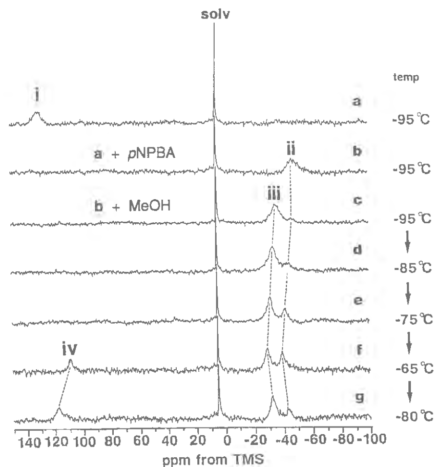
Figure 5. Deuterium NMR spectra of (a) pyrrole- d_8 - 1b - m CB [ 3.0 \times 10^{-3} M]; (b) 2b prepared by the addition of 1.8 equiv of p NPBA to 1b - m CB; (c) 3b formed by the addition of 2 equiv of 2b in dichloromethane at -95^\circ\text{C} ; (d)-(f) temperature dependence of deuterium NMR spectra of solution (c) at -85^\circ\text{C} , -75^\circ\text{C} , and -65^\circ\text{C} ; (g) a NMR spectrum of solution (f) at -80^\circ\text{C} .
