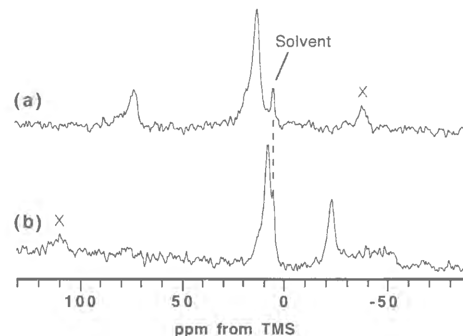
Figure 6. Deuterium NMR spectra of (a) pyrrole- d_8 - meta - d_8 - 1b - \text{ClO}_4 [ 1.0 \times 10^{-3} M] and (b) 3b' formed by the addition of 1.8 equiv of \text{F}_5\text{-PhIO} in dichloromethane containing 200 equiv of methanol at -90^\circ\text{C} . In (a), the signal at \sim 40 ppm is assigned to pyrrole \beta - ^2\text{H} of ferric low spin species.
