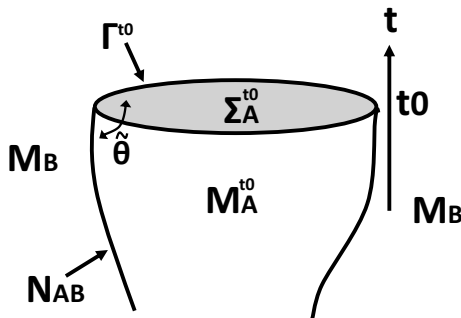
Figure 2. A sketch of Lorentzian gravity setup for the canonical formalism.
