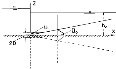
Fig. 1. Definition sketch of wall jet.
