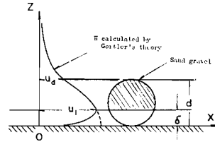
Fig. 22. Representative velocities in zone of established flow.
