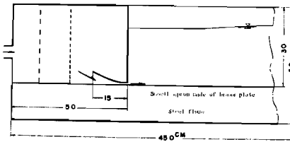
Fig. 2. Experimental apparatus.
