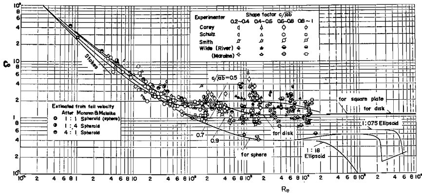
Fig. 16. Relation between drag coefficient of sphere and Reynolds number in comparison with other bodies'.
