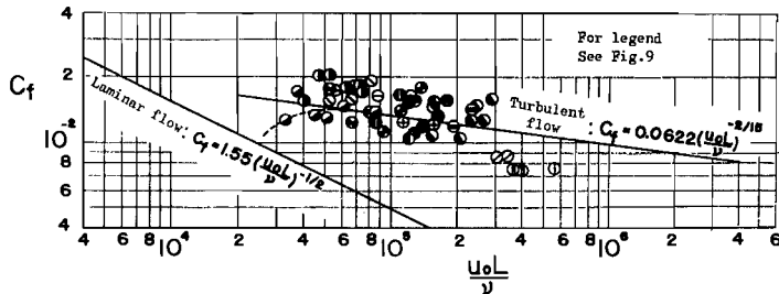
Fig. 23. Relation between C_f and u_0 L / \nu in region of \xi > 2\alpha^2 .
