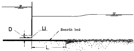
Fig. 13. Definition sketch of apron and flow downstream of submerged outlet.
