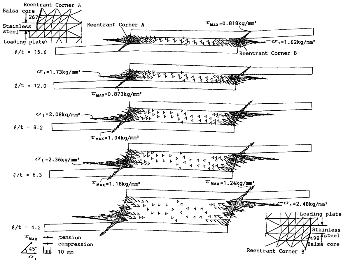
Fig. 3. Distribution of principal stress \sigma_1 and shear stress \tau_{\max} in balsa core.
