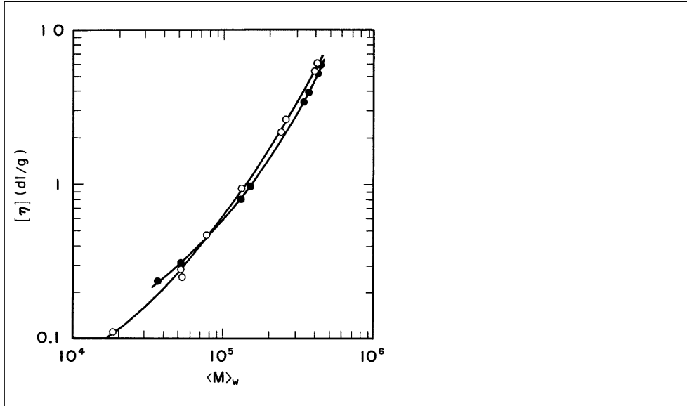
Fig. VI.13. Intrinsic viscosities of poly- \gamma -benzyl-L-glutamates (PBLG) in dimethylformamide at 25 °C. 106, 107 Open circles: PBLG-A (straight rods). Filled circles: PBLG-B (once-broken rods).
