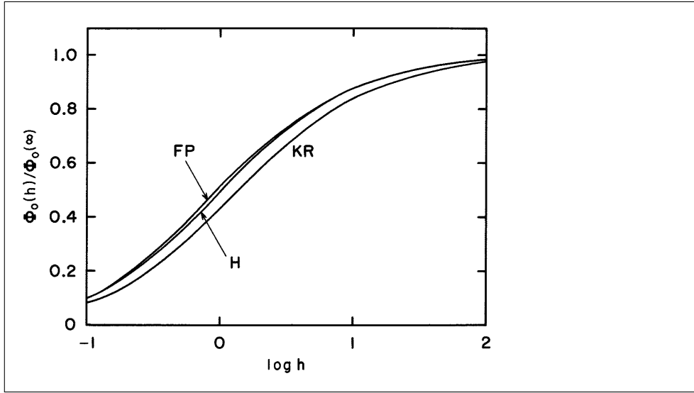
Fig. VI.4. The ratio \Phi_0(h)/\Phi_0(\infty) plotted against \log h . Curve KR: the Kirkwood–Riseman theory. Curve H: Hearst's version of the Zimm theory. Curve FP: the Fixman–Pyün theory.
