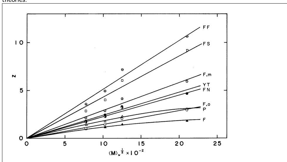
Fig. VII.14. Test of the linearity between z and (M_w)^{1/2} with data for polystyrene in toluene at 12^\circ\text{C} . 2 The values of z were calculated from various theories of \alpha_S ; \ominus , from the FF theory; \square , from the FS theory; \diamond , from the F,m theory; \bullet , from the YT theory; \ominus , from the FN theory; \circ , from the F,o theory; \triangle , from the P theory; \blacktriangle , from the F theory.
