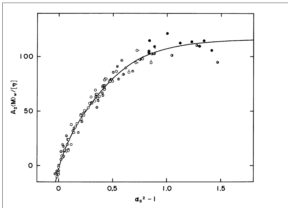
Fig. VII.17. Plots of A_2 \langle M \rangle_w / [\eta] against \alpha_s^2 - 1 for fractions of polychloroprene 27, 28 in carbon tetrachloride at 25 °C (●), n -butyl acetate at 25 °C (○), and trans -decalin at various temperatures (⊕), and for fractions of poly- p -methylstyrene 29 in toluene at 30 °C (●), dichloroethane at 30 °C (⊕), cyclohexane at 30 °C (○), methyl ethyl ketone at 30 °C (⊙), and diethyl succinate at various temperatures (○). The curve is an empirical fit to the data.
