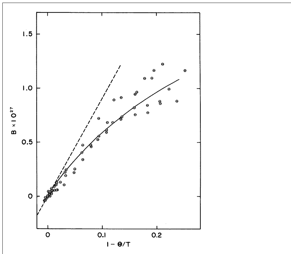
Fig. VII.16. Plots of B against 1 - \Theta/T for fractions of polystyrene in decalin. 2 The values of B were calculated from values of \alpha_S by the use of Eq. (40.8) with (39.6). The full curve is an empirical fit to the data. The broken line represents the temperature dependence of B determined by Berry from second virial coefficients.
