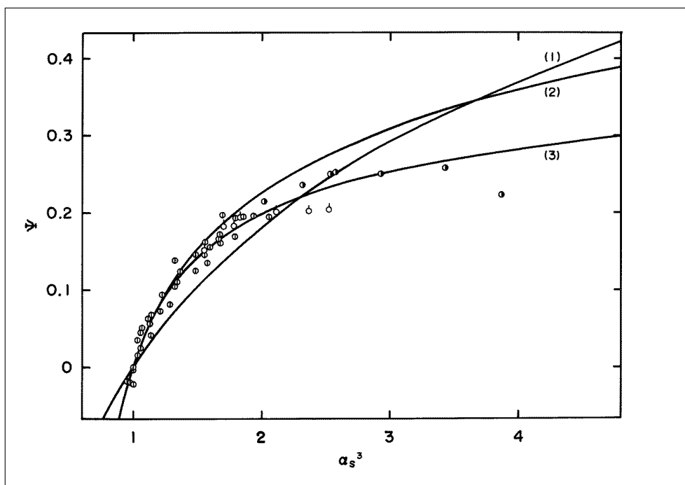
Fig. VII.12. Plots of \Psi against \alpha_S^3 for fractions of polychloroprene; 27 \bullet , in carbon tetrachloride at 25 °C; \circ , in n -butyl acetate at 25 °C; \odot , in trans -decalin at various temperatures. The curves have the same significance as those in Fig. VII.11.
