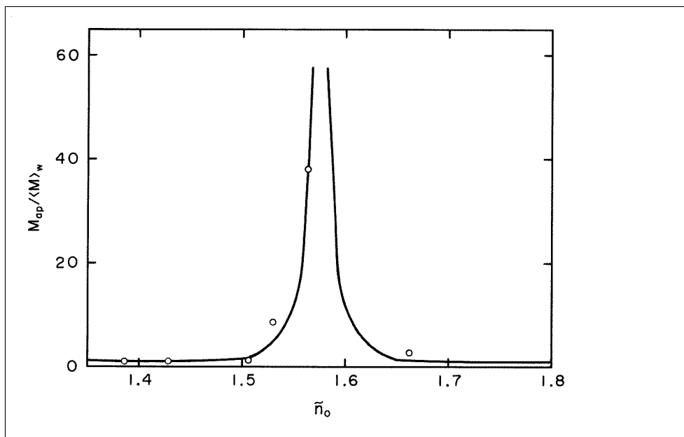
Fig. V.9. M_{ap}/\langle M \rangle_w plotted against \tilde{n}_0 for a mixture of 65% polystyrene and 35% polymethylmethacrylate. 47 Open circles: experimental data. The curves represent the values calculated from Eq. (28.48)
