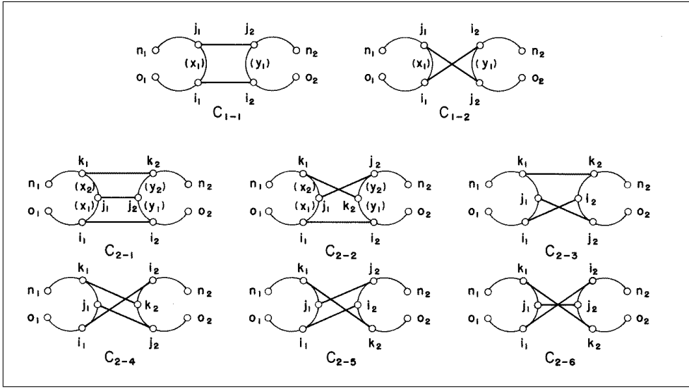
Fig. IV.1. Cluster diagrams for the double and triple intermolecular contact terms. The heavy lines connect the contact segments.
