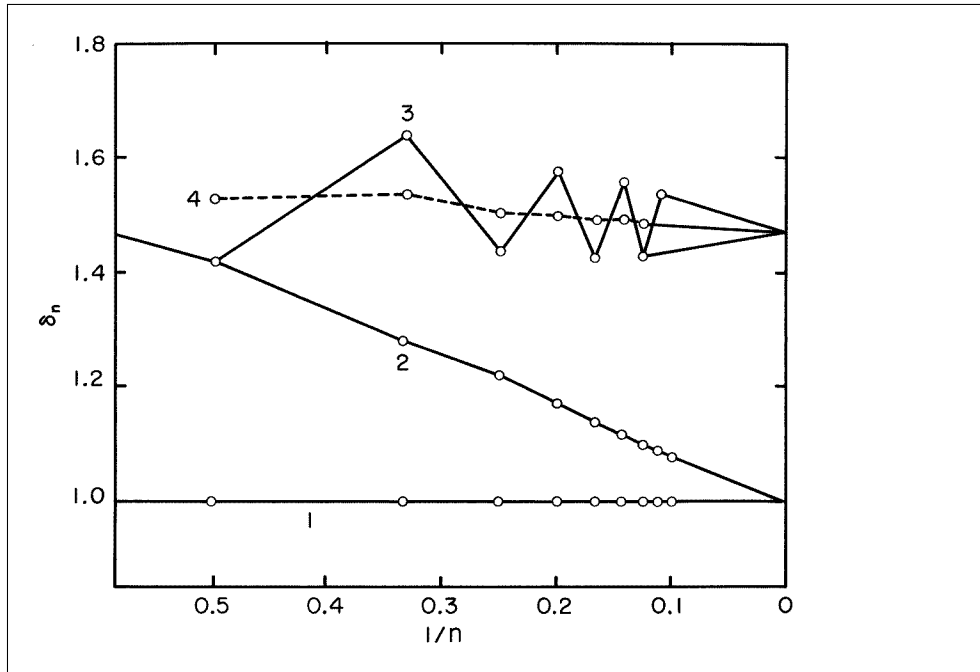
Fig. III.7. Successive estimates of \delta for two-dimensional square lattice chains. 68 1: completely random-flight chains. 2: chains only with immediate reversals forbidden. 3: three-choice, nonintersecting chains. 4: sequence of the means \frac{1}{2}(\delta_n + \delta_{n+1}) for case 3.
