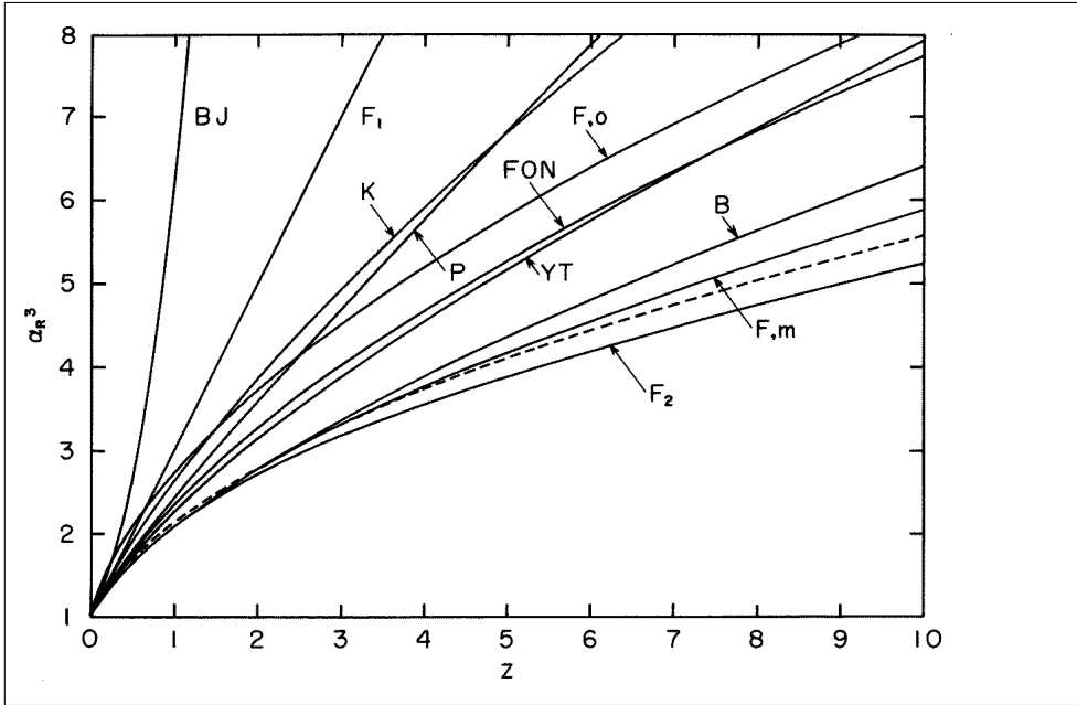
Fig. III.5. Theoretical values of \alpha_R^3 calculated from various approximate theories. Curve BJ: the Bueche–James theory, Eq. (15.19). Curve F_1 : the Fixman theory, Eq. (15.53). Curve P: the Ptitsyn theory, Eq. (15.61). Curve K: the Kurata theory, Eq. (15.41). Curve F_0 : the original Flory theory, Eq. (14.39). Curve FON: the Fujita–Okita–Norisuye theory, Eq. (15.44). Curve YT: the Yamakawa–Tanaka theory, Eq. (15.94). Curve B: the Bueche theory, Eq. (15.46). Curve F_m : the modified Flory theory, Eq. (14.40). Curve F_2 : the boson representation theory of Fixman. Broken curve: Eq. (15.96).
