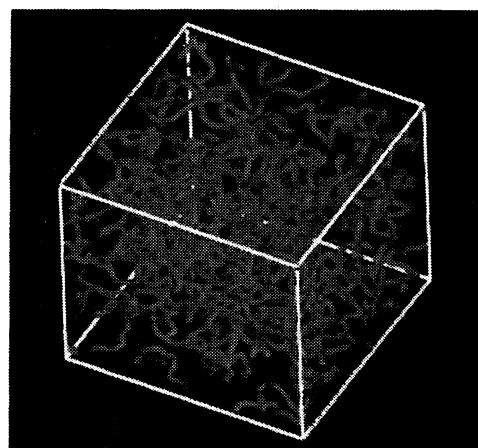
Fig.2 Quantum turbulence. The lines show the cores of quantized vortices.
