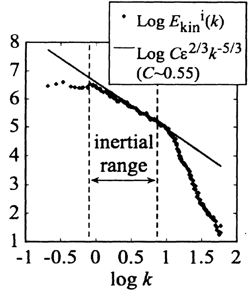
Fig.7 Energy spectrum E_{\text{kin}}^i(k) for the steady state QT. The points are from an ensemble average of 50 randomly selected states at t > 25 . The solid line is the Kolmogorov law. The inertial range corresponds to 2\pi/X_0 < k < 2\pi/\xi , in which the spectrum obeys the Kolmogorov law. The Kolmogorov constant C \approx 0.55 is lower than the usual value C \approx 1.4 , the reason of which is not known.
