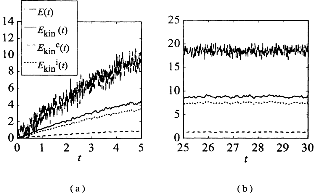
Fig.5 Results of numerical simulation of the GP equation with energy injection at large scales and energy dissipation at small scales. Time development of the total energy E(t) , the kinetic energy E_{kin}(t) , the compressible kinetic energy E_{kin}^c(t) , and the incompressible kinetic energy E_{kin}^i(t) at (a) the initial stage and (b) a later stage. The system is found to be statistically steady at the later stage.
