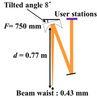
Fig. 4.19. Calculation model of the beam radius calculated from \omega_0 = 0.43 mm and d = 0.77 m .
