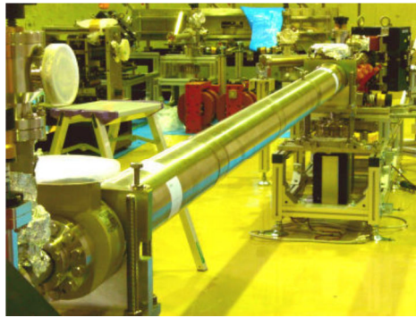
Fig. 3.10. The photograph of the accelerator tube used in the KU-FEL.
