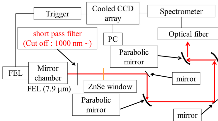
Fig. 4.32. Schematic of the experimental setup.
