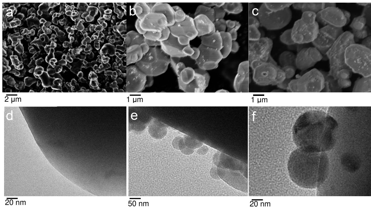
Fig. 2. (a-c) SEM and (d-f) TEM images of the prepared samples; (a,d) CTO, (b, e,f) Ag(PD)/CTO, and (c) Ag(PD)-NiO x (PD)/CTO.
