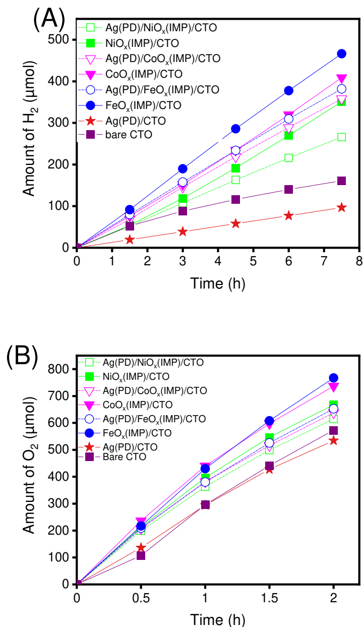
Fig. 7. [A] Time course of H 2 evolution from an aqueous methanol solution with different single and dual cocatalyst loaded CTO photocatalyst samples; Ag(PD)/NiO x (IMP)/CTO, NiO x (IMP)/CTO, Ag(PD)/CoO x (IMP)/CTO, CoO x (IMP)/CTO, Ag(PD)/FeO x (IMP)/CTO, FeO x (IMP)/CTO, Ag(PD)/CTO and bare CTO, where methanol was used as an electron donor. [B] Time course of O 2 evolution test from an aqueous solution of NaIO 3 with the photocatalyst samples; Ag(PD)/NiO x (IMP)/CTO, NiO x (IMP)/CTO, Ag(PD)/CoO x (IMP)/CTO, CoO x (IMP)/CTO, Ag(PD)/FeO x (IMP)/CTO, FeO x (IMP)/CTO, Ag(PD)/CTO and bare CTO, where NaIO 3 was used as electron acceptor.
