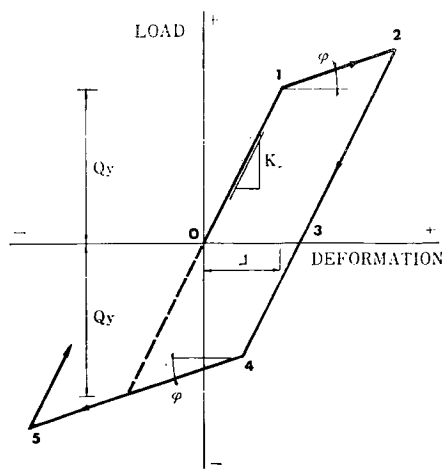
Fig. 5 Load-deformation Relations for Jenkin's Model
