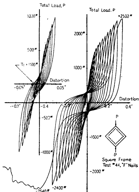
Fig. 3 Experimental Record of Load-distortion for a Hinged Square Frame Stiffened by Two Plywood Panels
