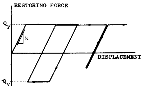
Fig. 1(b) Force-displacement Relations
