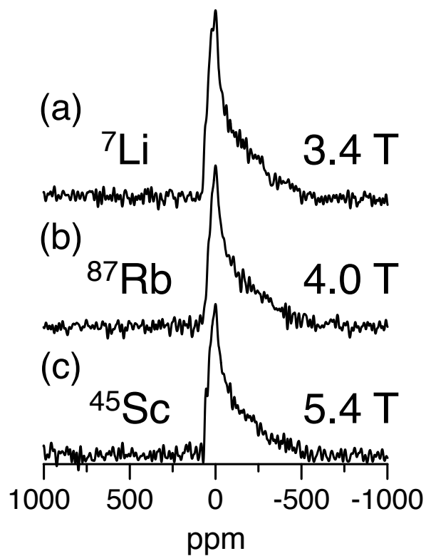
Fig. 4. NMR spectra of (a) {}^7\text{Li} , (b) {}^{87}\text{Rb} , and (c) {}^{45}\text{Sc} nuclei in aqueous solution of a mixture of \text{LiCl} , \text{RbCl} , and \text{ScCl}_3 measured in magnetic fields of 3.4, 4.0, and 5.4 T, respectively. No shimming was performed.
