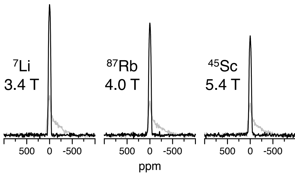
Fig. 7. ^7\text{Li} , ^{87}\text{Rb} , and ^{45}\text{Sc} spectra obtained using the paramagnetic shim pellets with the optimized configuration. For comparison, the spectra obtained without shimming are shown in the gray lines. The number of scans was 8000 for each spectrum.
