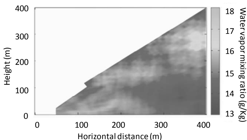
Figure 1. Distribution of water vapor mixing ratio in a vertical plane over Shigaraki at 22:17 JST on August 28, 2012.
