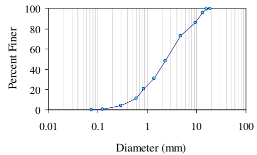
Fig. 6 Particle size distribution of bed sediment
