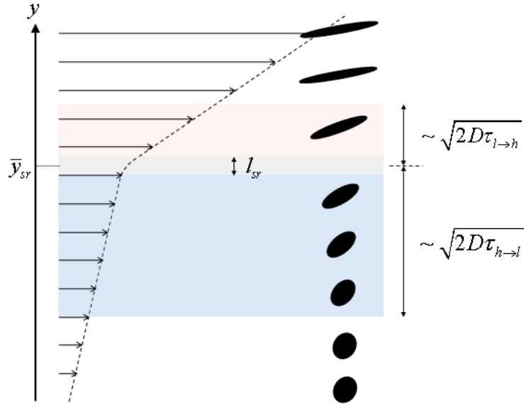
Fig. 5. Schematic diagram showing competition of molecular diffusion and relaxation. l_{sr} and l_{mc} are the boundary widths for the shear rate and conformation bands, respectively. \tau_{h\rightarrow l} and \tau_{l\rightarrow h} are the characteristic relaxation times of molecular conformation on a switch of local shear rate, from \dot{\gamma}_{high} to \dot{\gamma}_{low} and from \dot{\gamma}_{low} to \dot{\gamma}_{high} , respectively.
