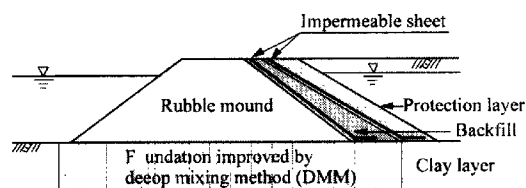
c) Rubble mound type quay wall
