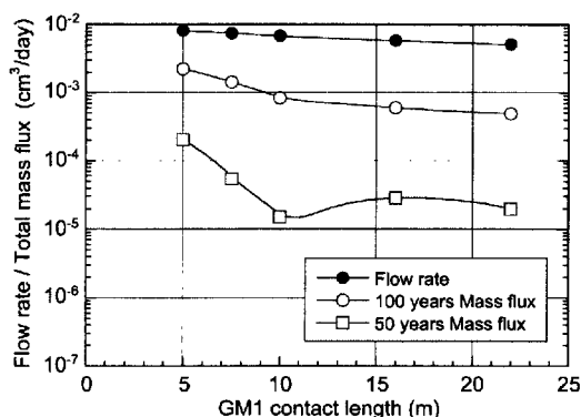
Fig. 16 Total mass flux affected by GM1 contact length
