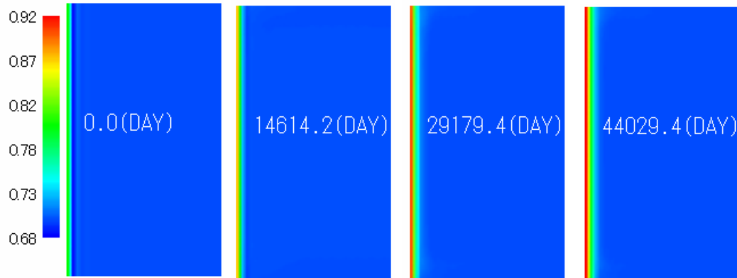
Figure 6.14 Distribution of degree of saturation (%)
