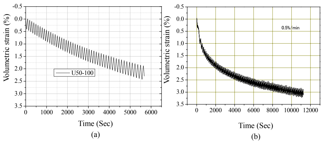
Figure 4.30 Volumetric vs. time: (a) simulated results and (b) experimental results
