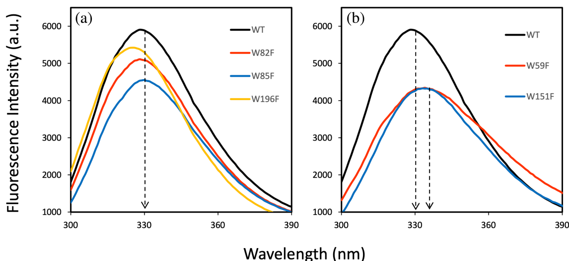
FIGURE 2 Intrinsic Trp fluorescence of \beta B2 WT and its mutants. (a) WT is shown in black; W82F is shown in red; W85F is shown in blue; W196F is shown in yellow. (b) WT is shown in black; W59F is shown in red; W151F is shown in blue. W151F and W59F have the lowest Trp fluorescence intensities, and they exhibit a right-shift pattern, indicating partial unfolding of the \beta B2 structure. WT, wild type.
