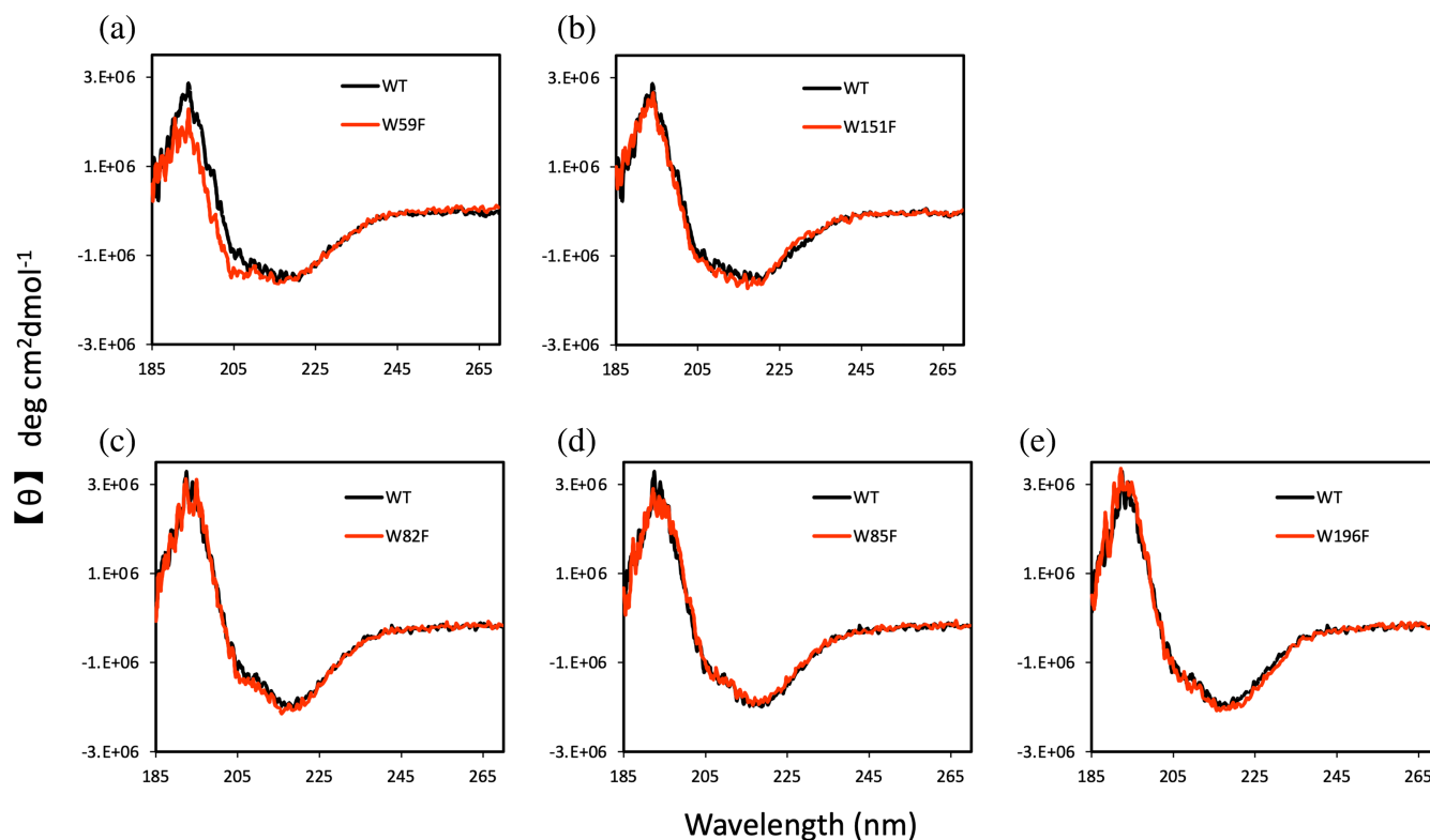
FIGURE 1 Comparison of \beta B2 secondary structures among mutants. WT is shown in black, and the mutants are shown in red. (a) W59F has a left-shift on its CD pattern indicating potential disorders on the Greek key Motifs. (b–e) W151F, W82F, W85F, and W196F bear no differences in secondary structure compared to WT. CD, circular dichroism; WT, wild type.
