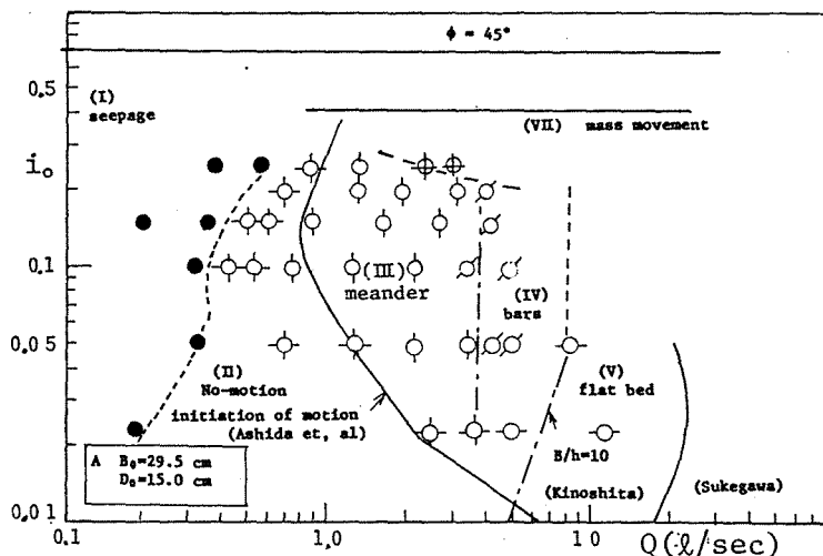
Fig. 1.3(a) Channel Pattern of Uniform Gravel
