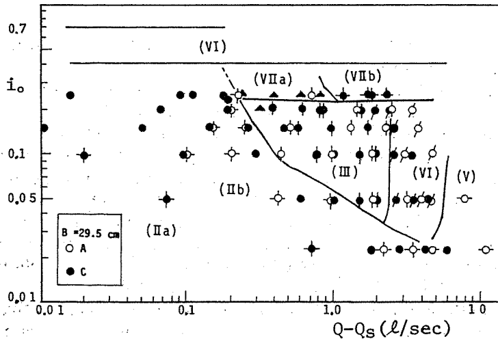
Fig. 1.4 Channel Patterns
