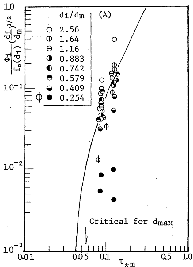
Fig. 4.14 Bed Load Transport Rate in the Beginning of Water Supply
