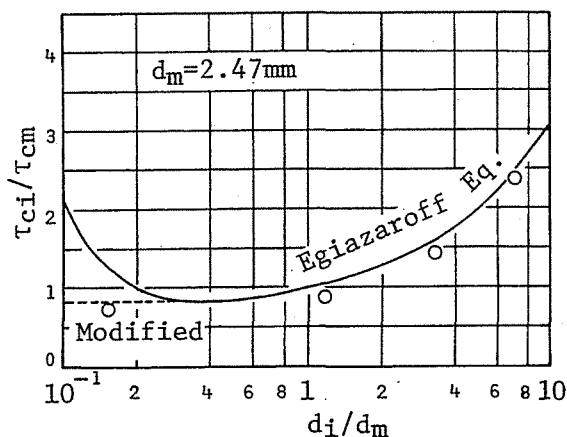
Fig. 3.2 Critical Tractive Force for Gravel Particles of Different Diameters
