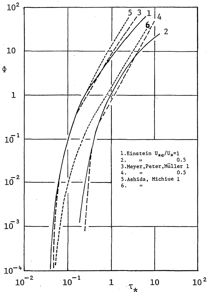
Fig. 4.1 Bed Load Equations
