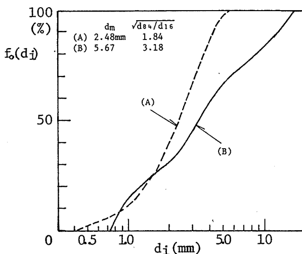
Fig. 4.12 Grain Size Distribution of Sand Materials used in the Experiments
