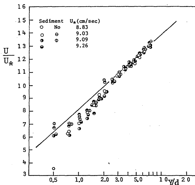
Fig. 1.13 Velocity Distribution of Flow with Sediment and without Sediment
