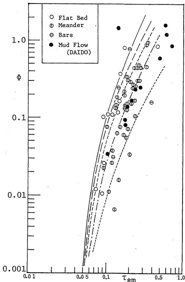
Fig. 1.12 Sediment Transport Rate
