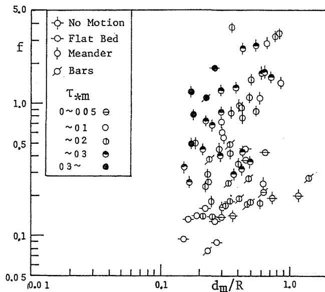
Fig. 1.11 Resistance Coefficient
