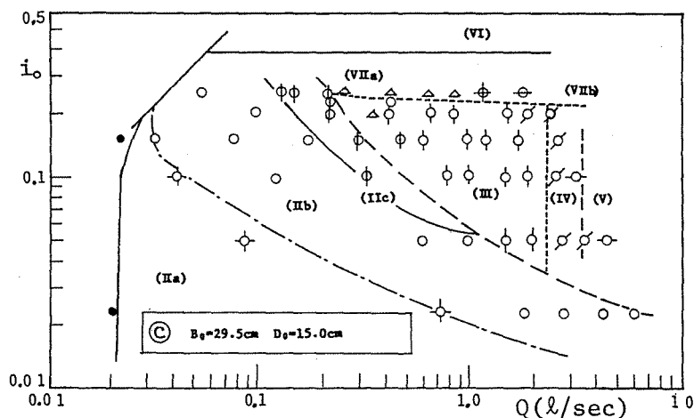
Fig. 1.3(b) Channel Pattern of Gravel Mixture
