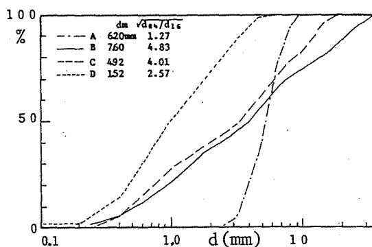
Fig. 1.1 Grain Size Distribution for Four Types of Sand used in the Experiments
