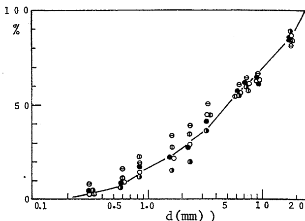
Fig. 4.11 Grain Size Distribution of Bed Material and That of Bed Load
