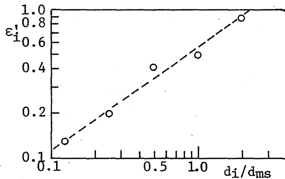
Fig. 3.21 The Relationship between \epsilon_i^1 and d_i/d_{ms}
