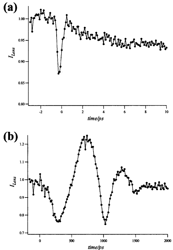
FIG. 3. The TrL signals after irradiation of focused fs-laser pulse inside a silicate glass, (a) in a short-time range, and (b) in a long-time range. The power of the pump beam was 1.45 \mu\text{J/pulse} , and the polarization of the pump and probe was perpendicular. The signals were normalized by the light intensity without the pump pulse. Upper direction indicates the creation of the convex lens.
