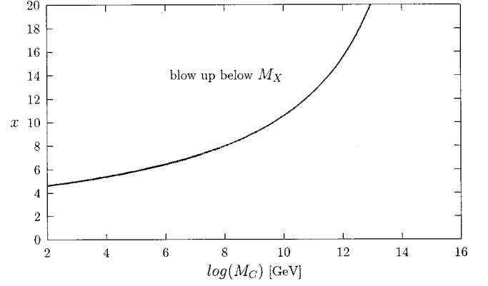
FIG. 1. Blowup of g_3 .
