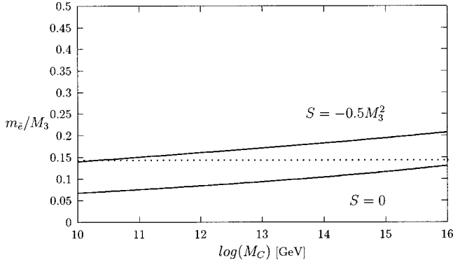
FIG. 6. m_{\tilde{e}}/M_3 for S=0 and -0.5M_3^2 .
