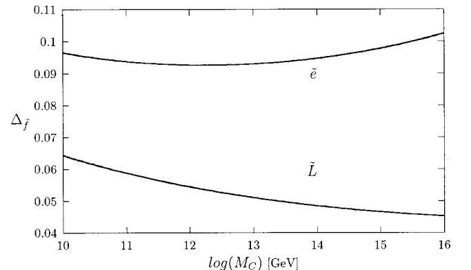
FIG. 3. \Delta_{\tilde{L}} and \Delta_{\tilde{e}} against M_c .
