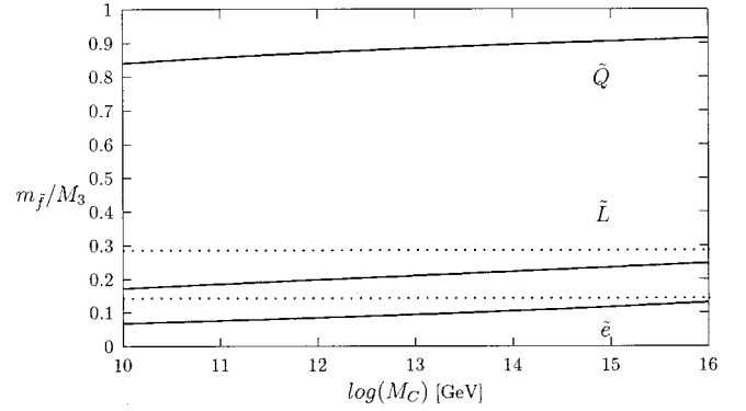
FIG. 5. Ratios of sfermion masses to M_3 at the weak scale. The three solid lines correspond to m_{\tilde{Q}}/M_3 , m_{\tilde{L}}/M_3 , and m_{\tilde{\epsilon}}/M_3 , respectively. The two dotted (upper and lower) lines correspond to ratios of gaugino masses to M_3 ( M_2/M_3 and M_1/M_3 ).
