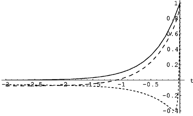
FIG. 7. The running couplings (y_1, M', A_\lambda) are shown in ratio to their initial values by a solid, a dashed, and a long-dashed line, respectively. t = \log_{10}(\mu/\Lambda_c) .
