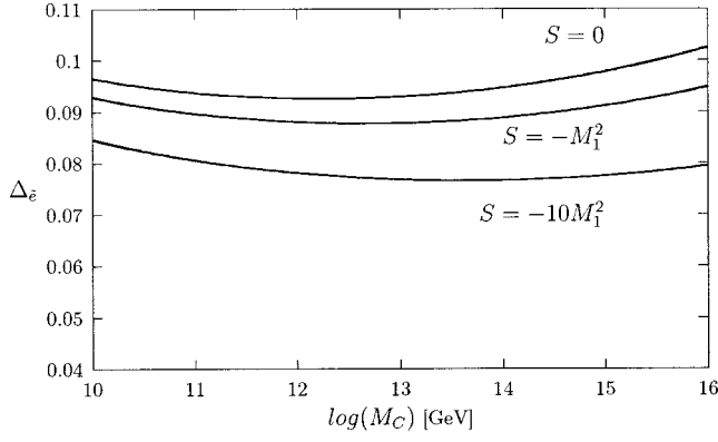
FIG. 4. \Delta_{\tilde{\epsilon}} against M_C with S=0 , S=-M_1^2 , and S=-10M_1^2 .
