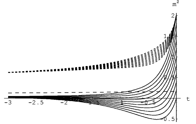
FIG. 8. RG flows for (m_1^2, m_Q^2 + m_P^2) shown by solid and dashed lines, respectively. The long-dashed line gives \alpha M^2 .
