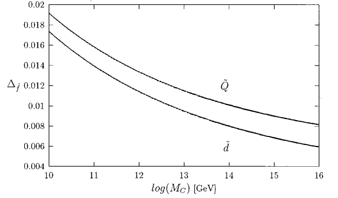
FIG. 2. \Delta_{\tilde{Q}} and \Delta_{\tilde{d}} against M_c .
