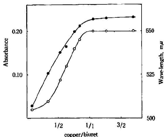
Fig. 2 Relations between the value of copper/biuret and absorption (wave-length and absorbance at their maxima)
